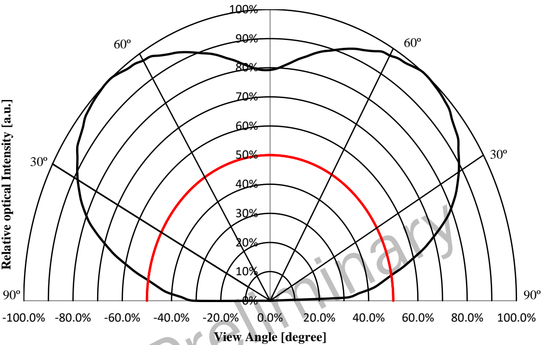
FIG 6. Far-field Emission Pattern
