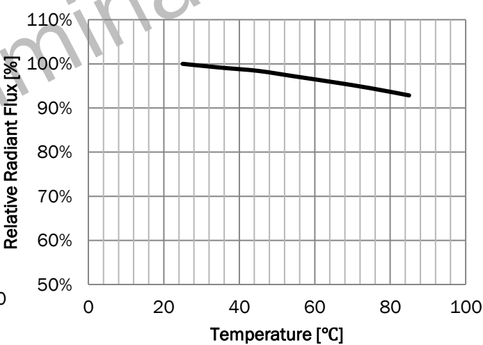
Fig 4. Relative Radiant Flux vs Ambient Temperature
